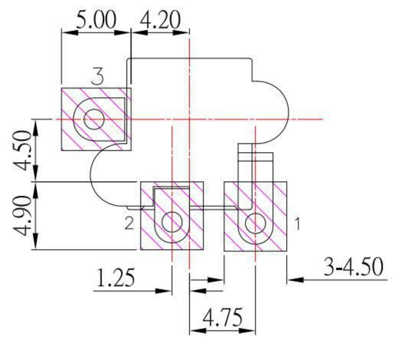
RECOMMENDED SOLDER PAD LAYOUT
