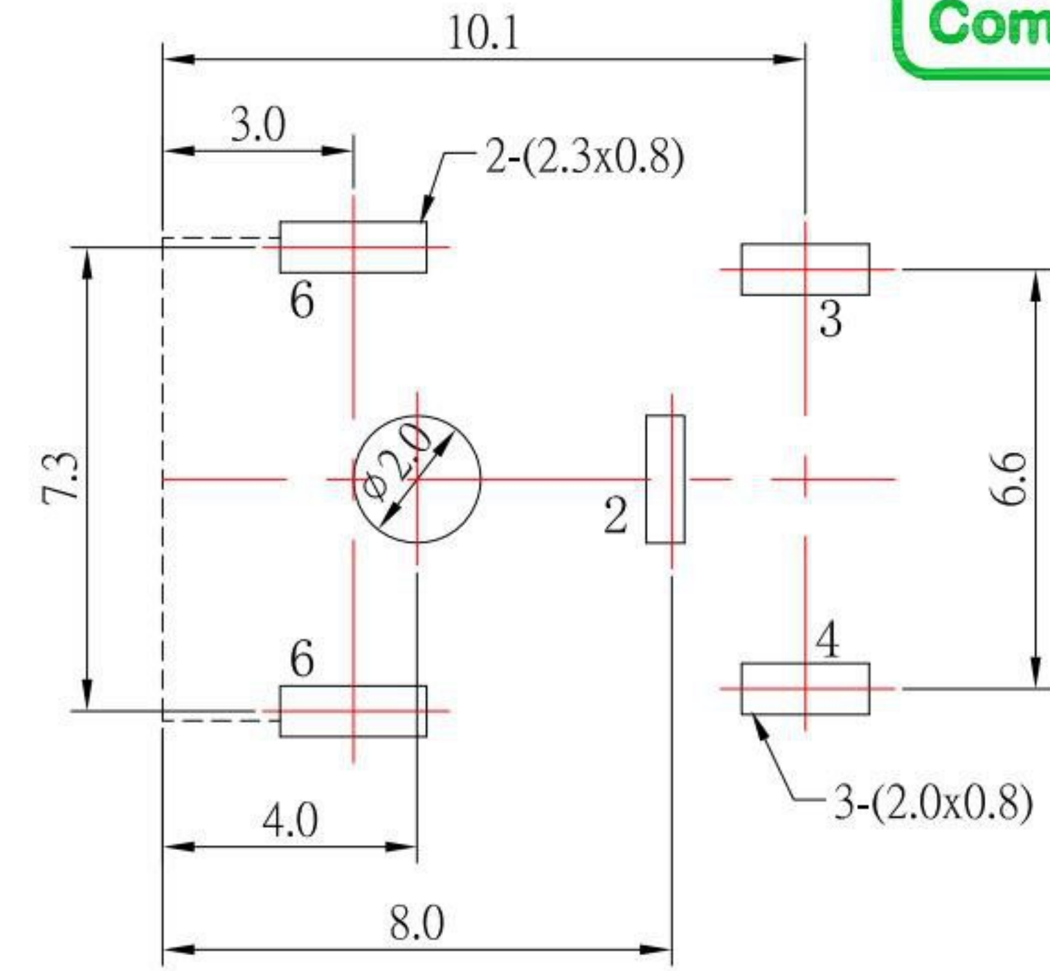
P.C.B LAYOUT MOUNTING PATTERN (TOP-VIEW)
