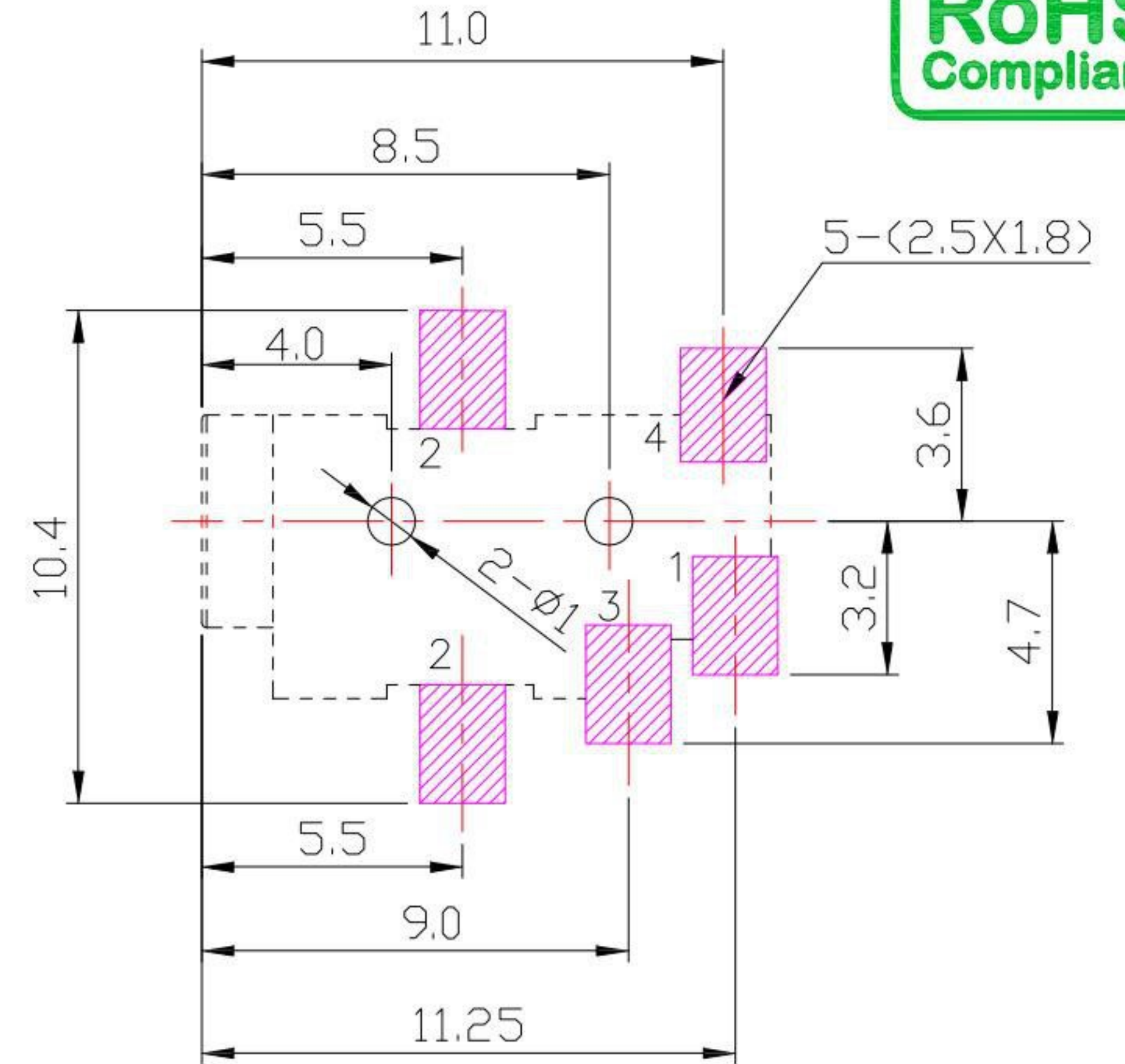
P.C.B LAYOUT TOP VIEW
