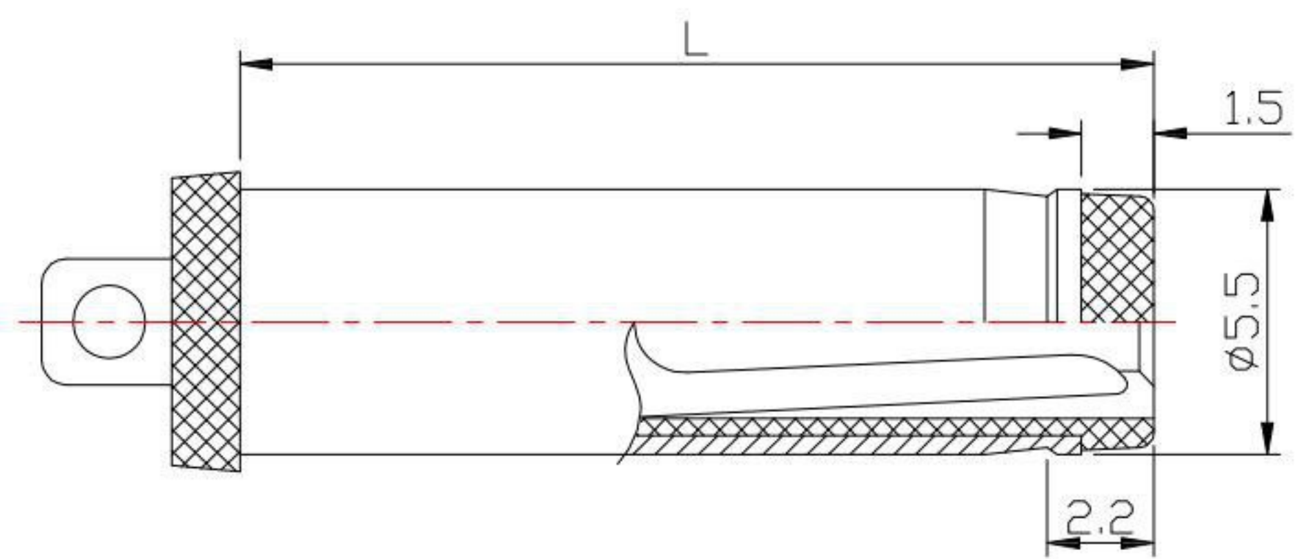
RECOMMENDED PLUG
