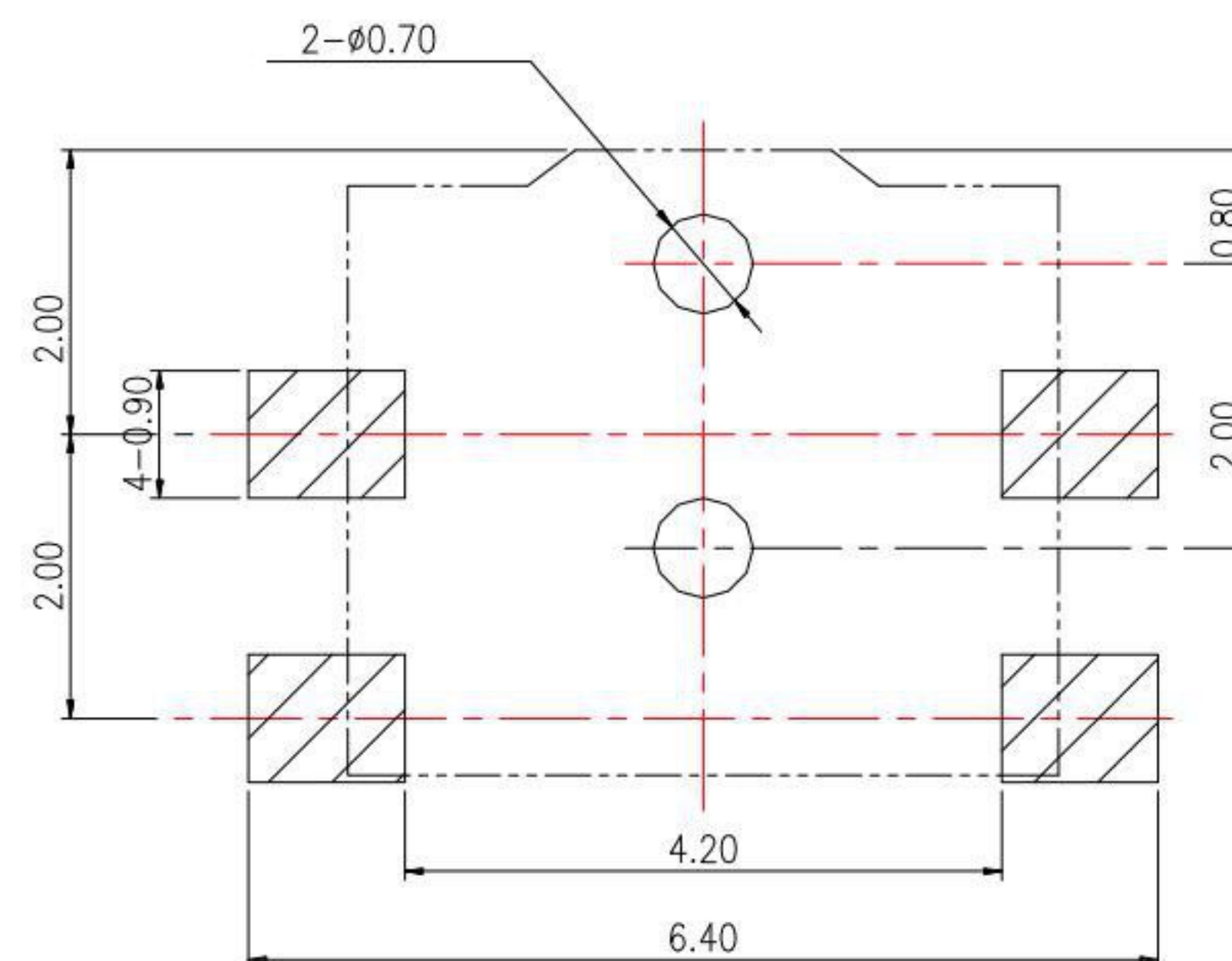
P.C.B. LAYOUT (VIEW FROM THE DIRECTION A)
