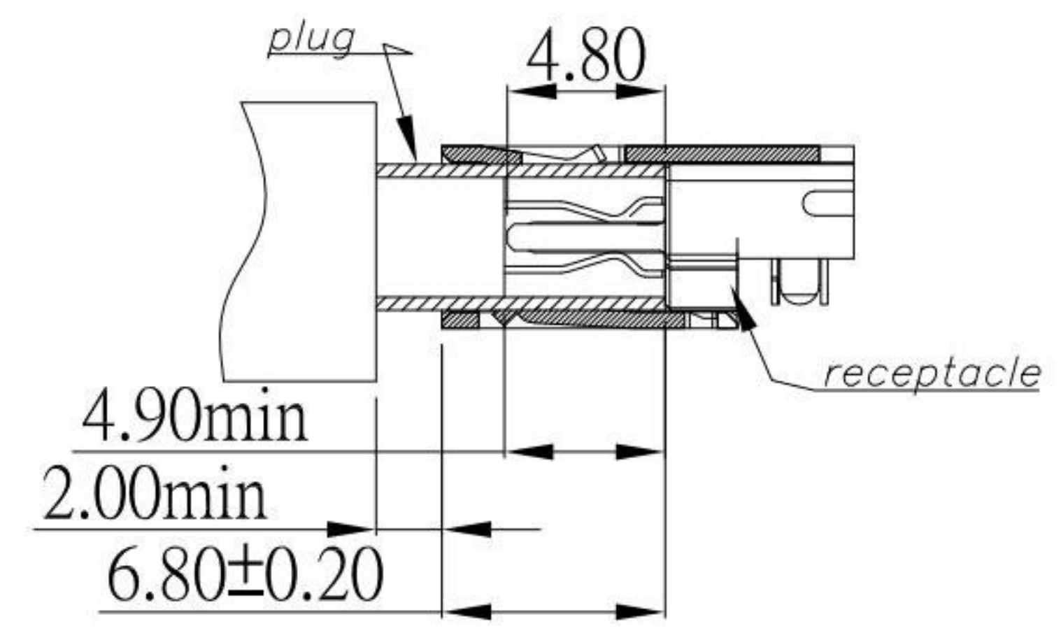
Mated Condition
