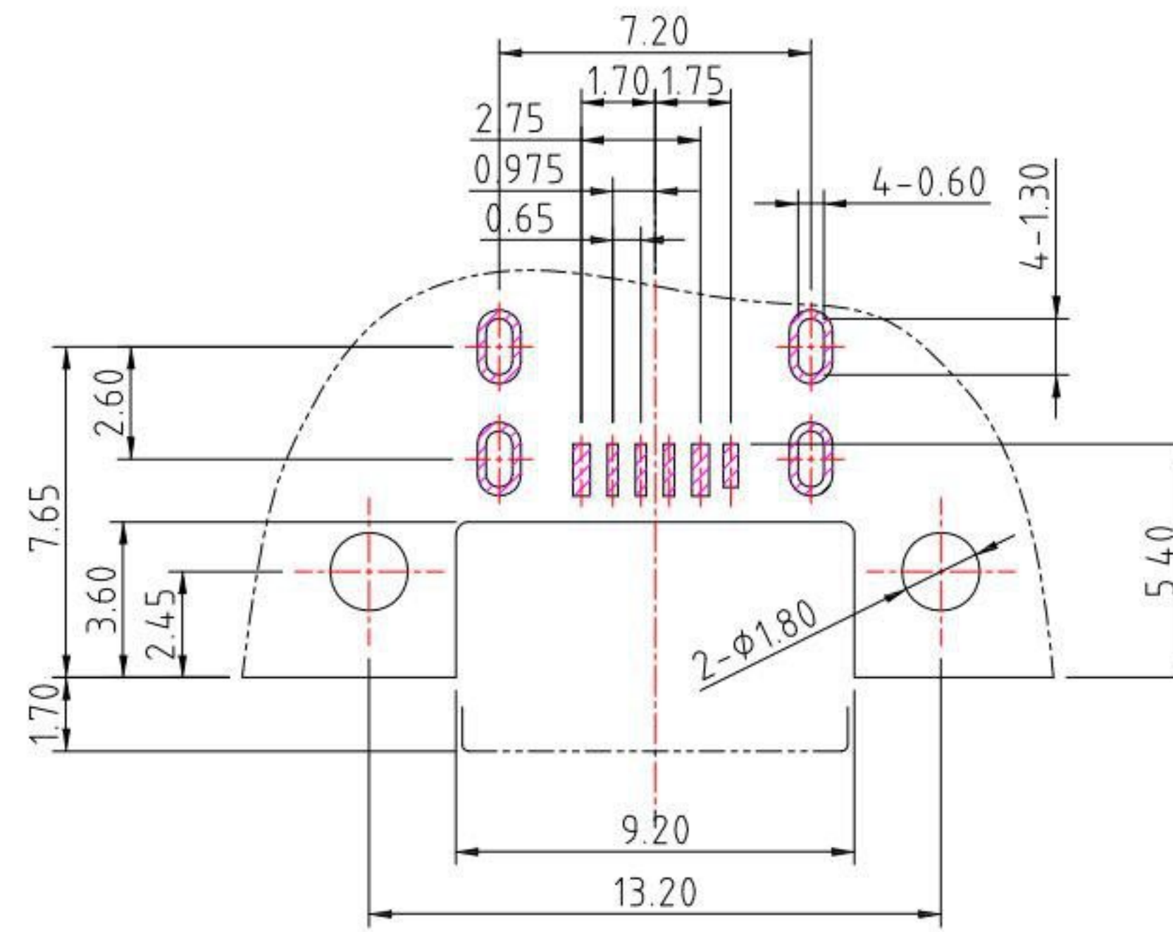
P.C.B LAYOUT MOUNTING PATTERN
