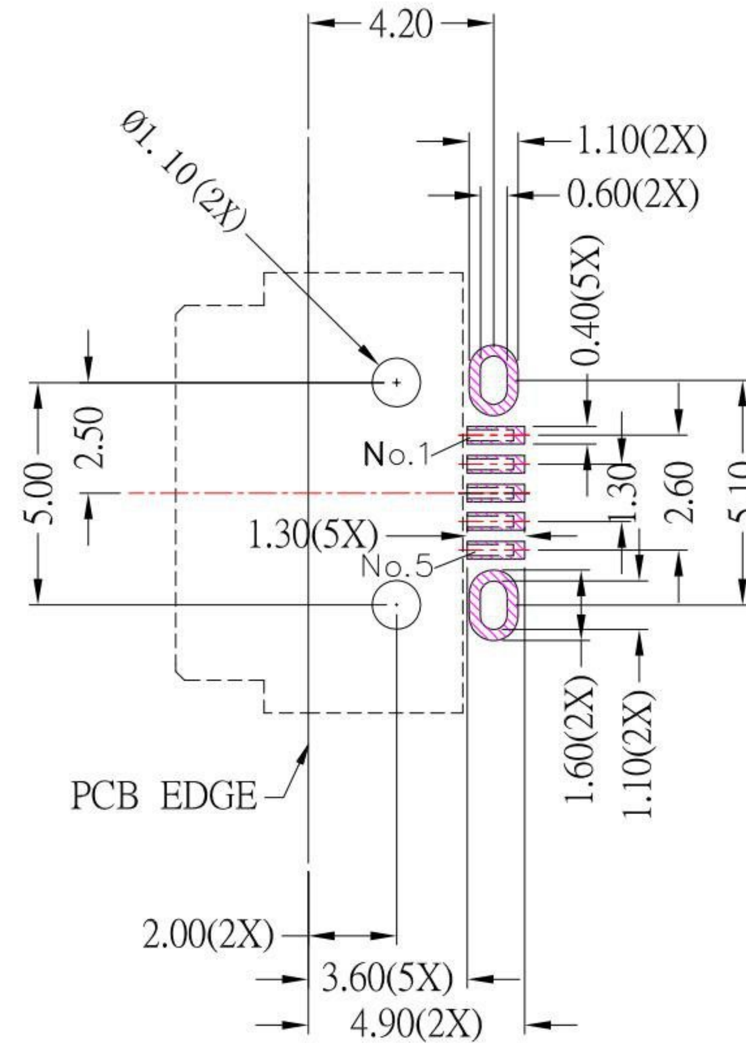
PCB LAYOUT MOUNTING PATTERN TOP VIEW
