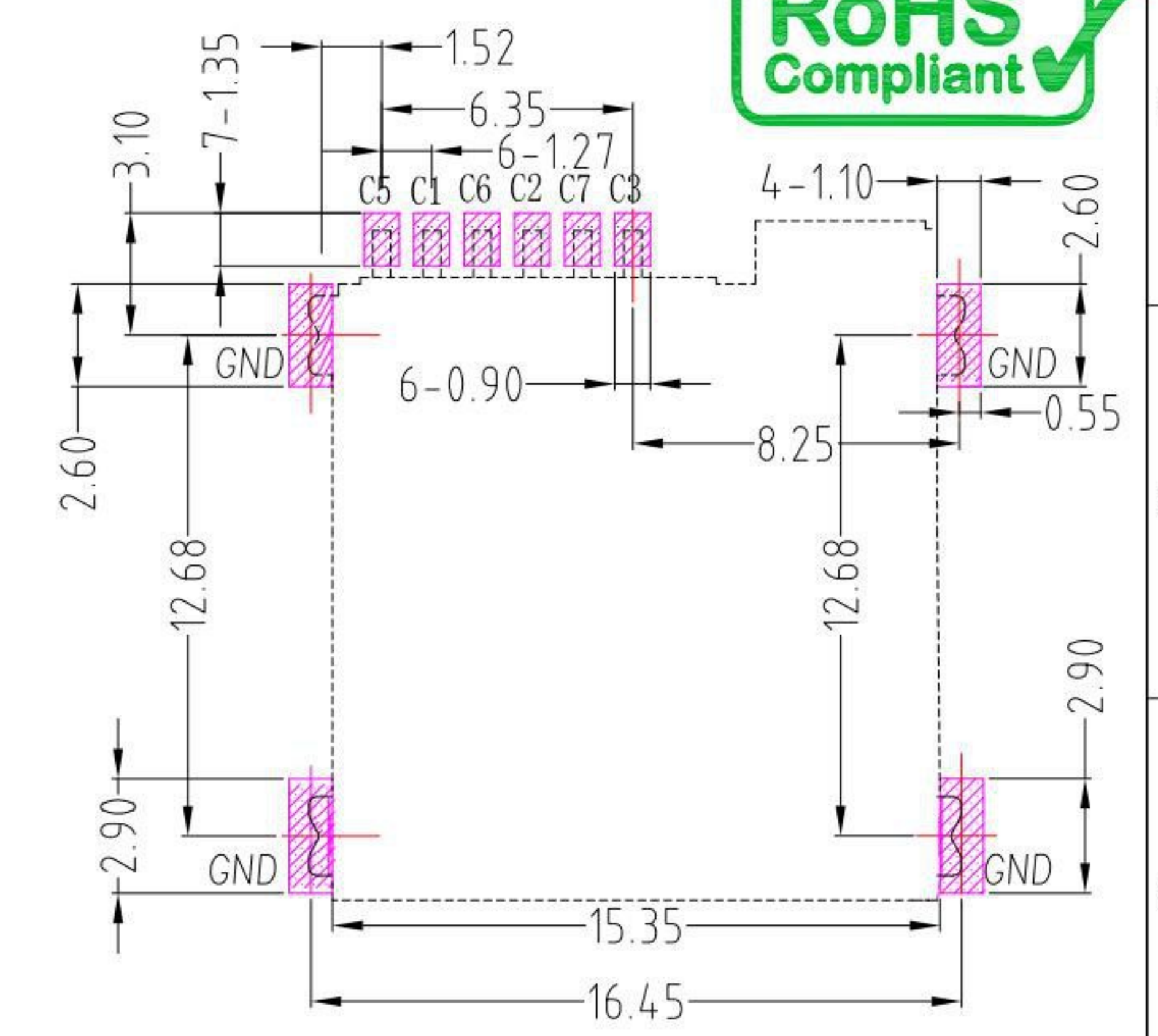
PCB LAYOYT
