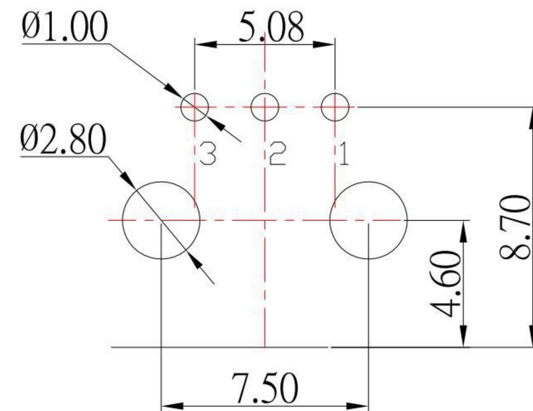
Recommended PCB Layout <BOTTOM VIEW>
