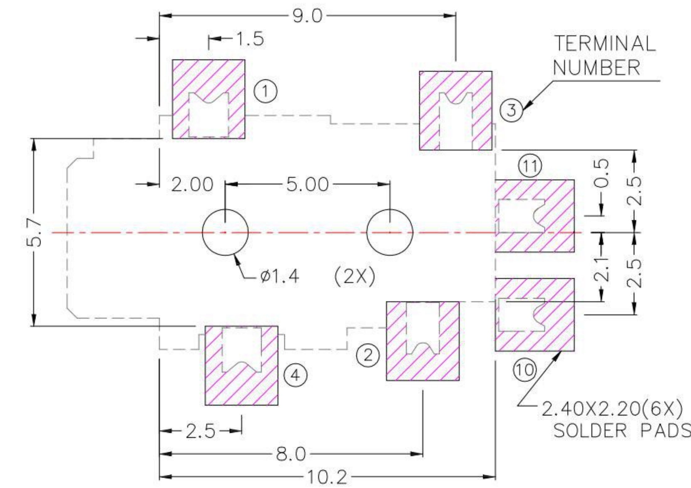
RECOMMENDED SOLDER PAD LAYOUT
