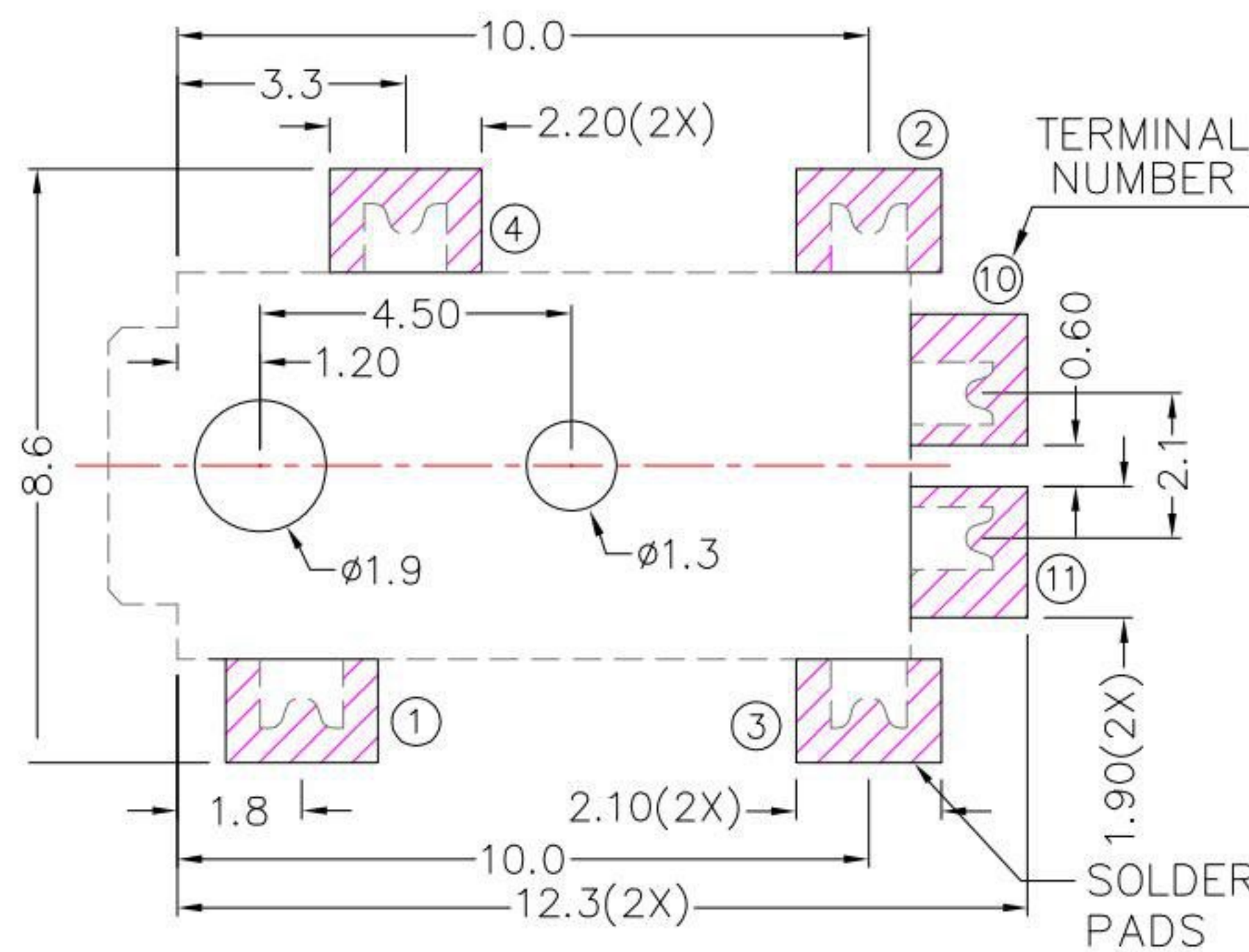
RECOMMENDED SOLDER PAD LAYOUT
