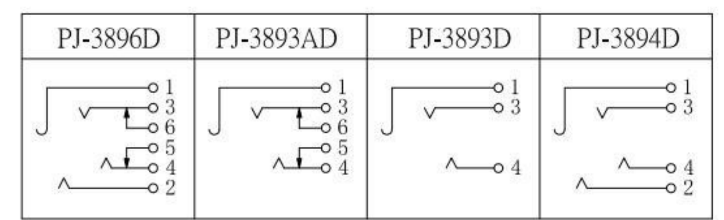
SCHEMATIC
