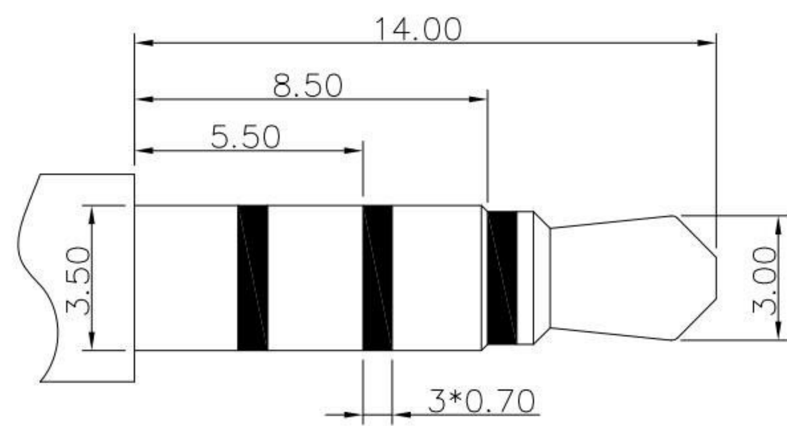
φ3.50mm 4 POLE PLUG
