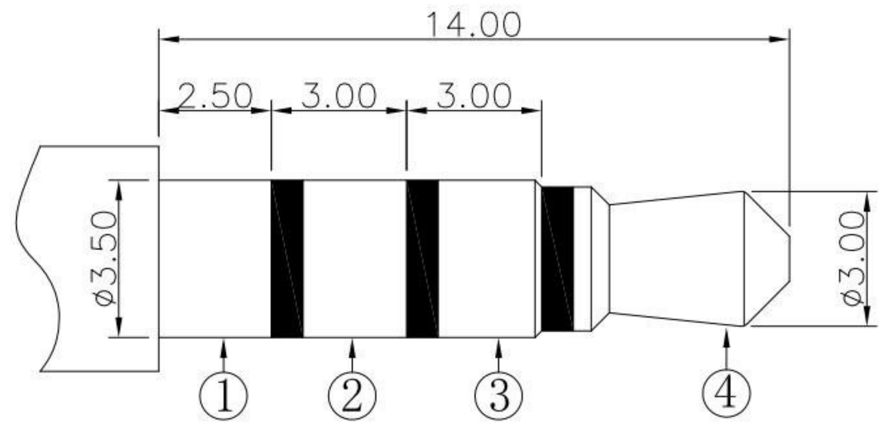
ø3.50mm 4 POLE PLUG
