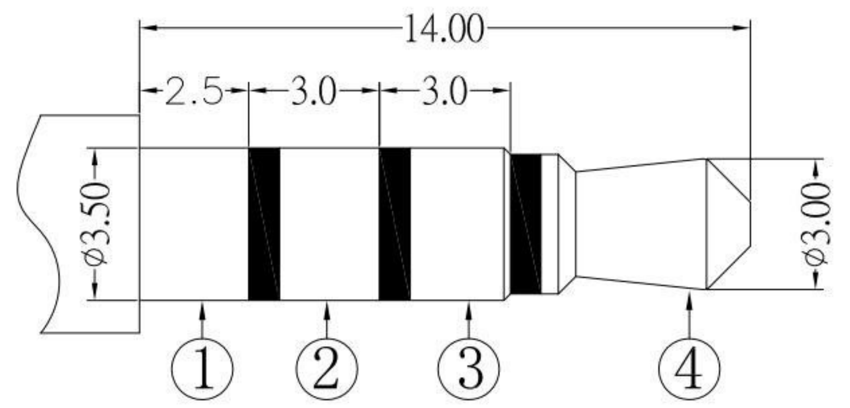
φ3.50mm 4 POLE PLUG
