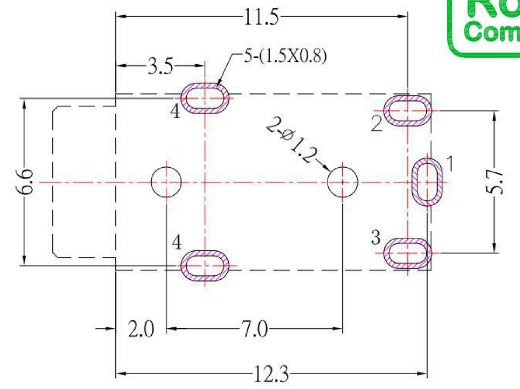
P.C.B LAYOUT MOUNTING PATTERN (TOP VIEW)
