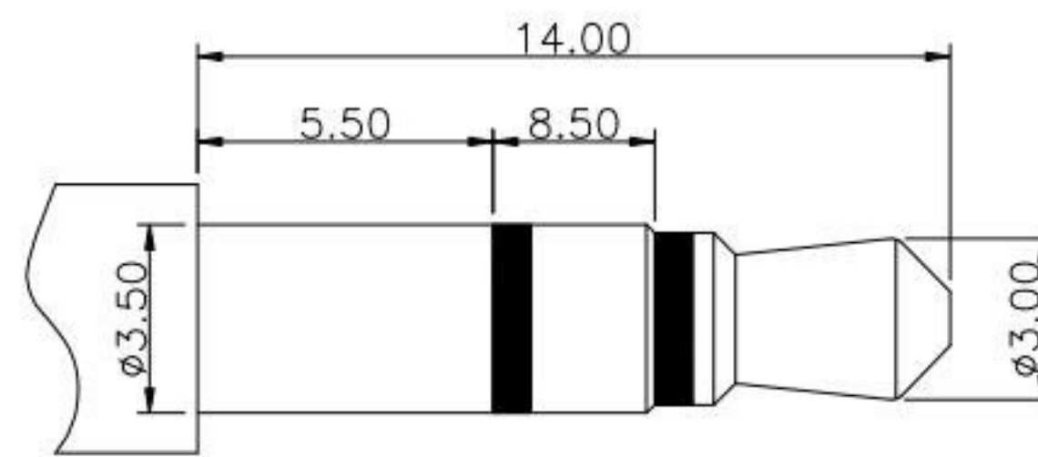
Ø3.50mm 3 POLE PLUG
