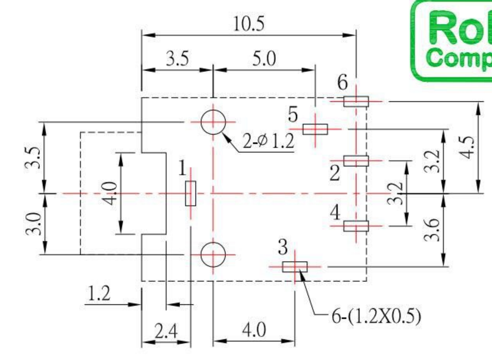
P.C.B LAYOUT TOP VIEW
