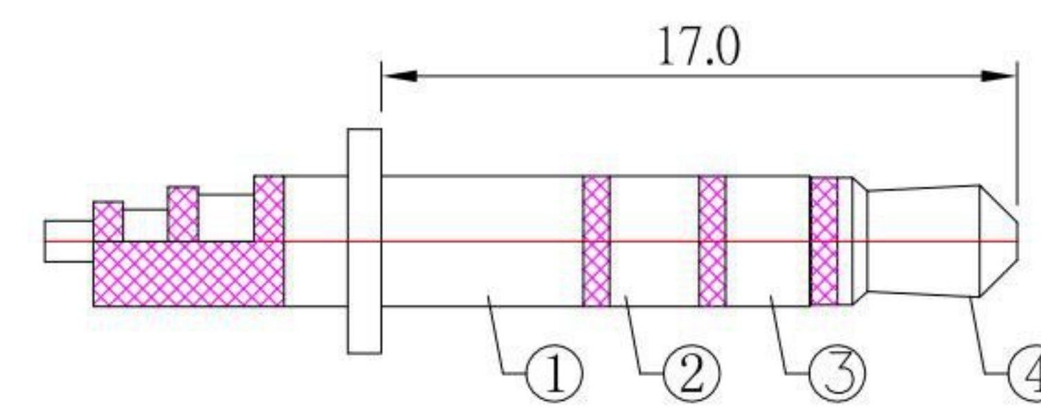
SCHEMATIC
