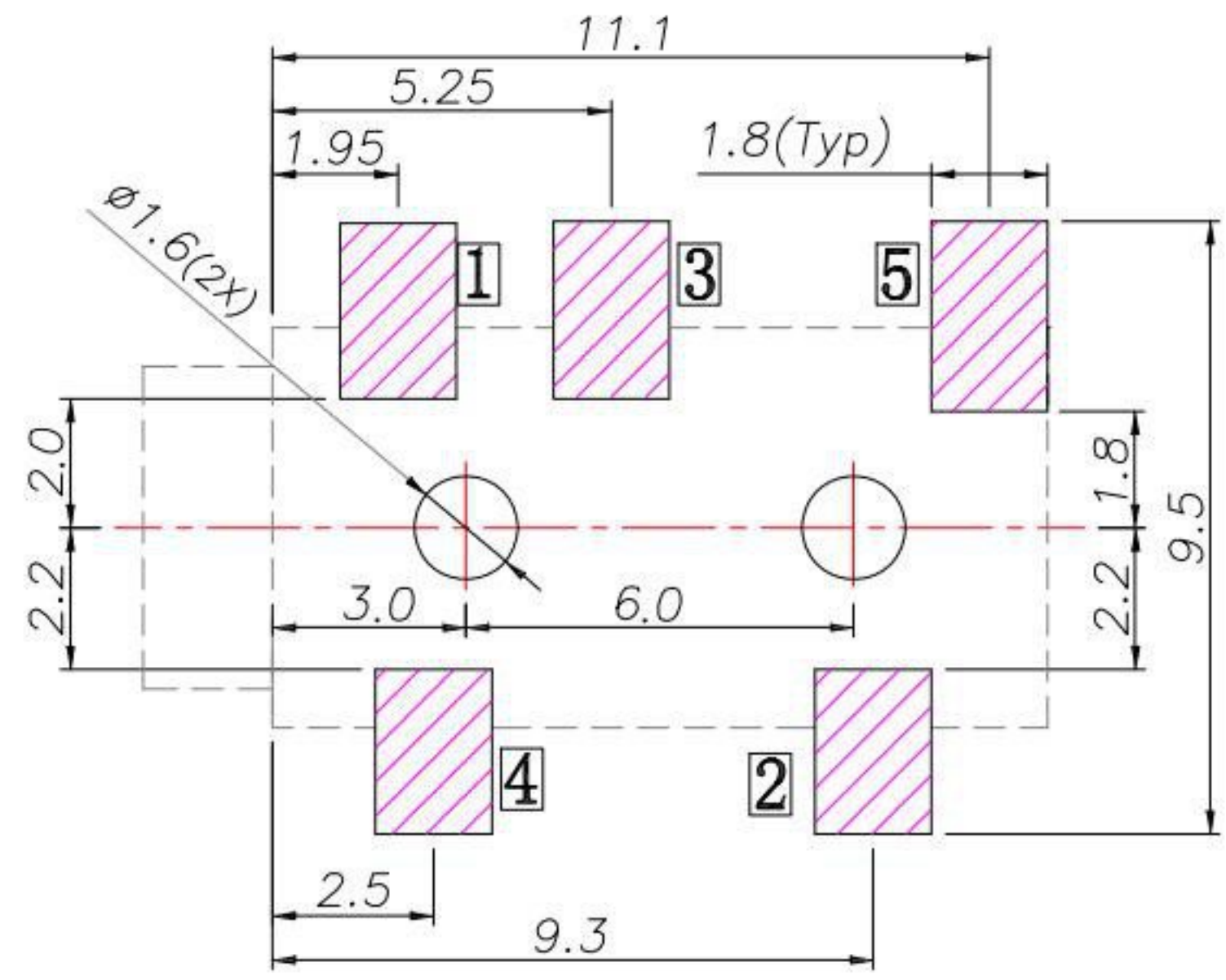
RECOMMENDED P. C. B. LAYOUT (COPPER-SIDED VIEW)
