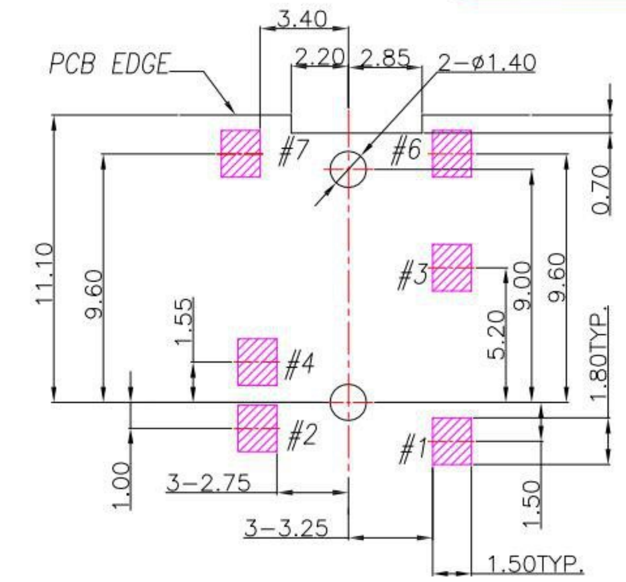
P.C.B LAYOUT MOUNTING PATTERN (TOP VIEW)
