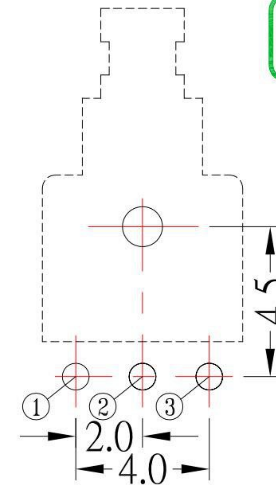
P.C.B. LAYOUT BOTTOM VIEW
