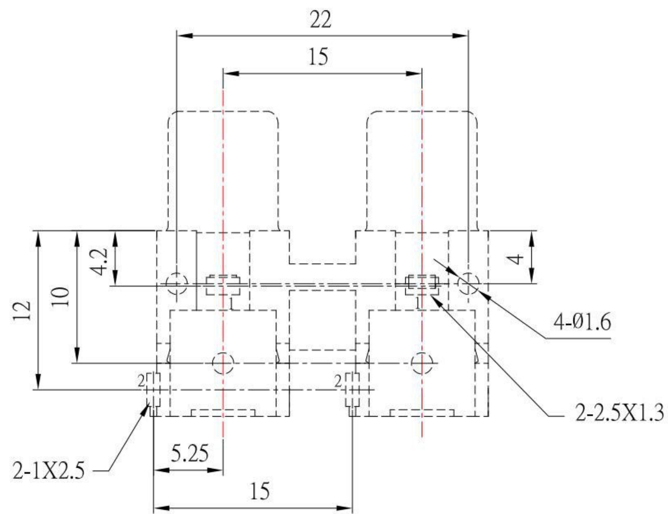
PCB HOLES DIAGRAM BOTTOM VIEW
