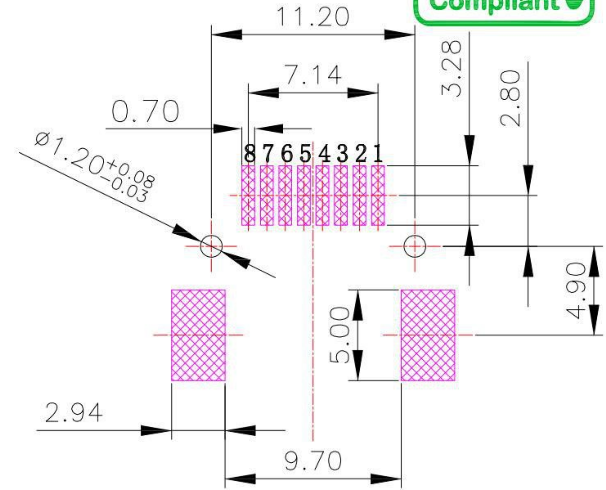
PCB LAYOUT MOUNTING PATTERN
