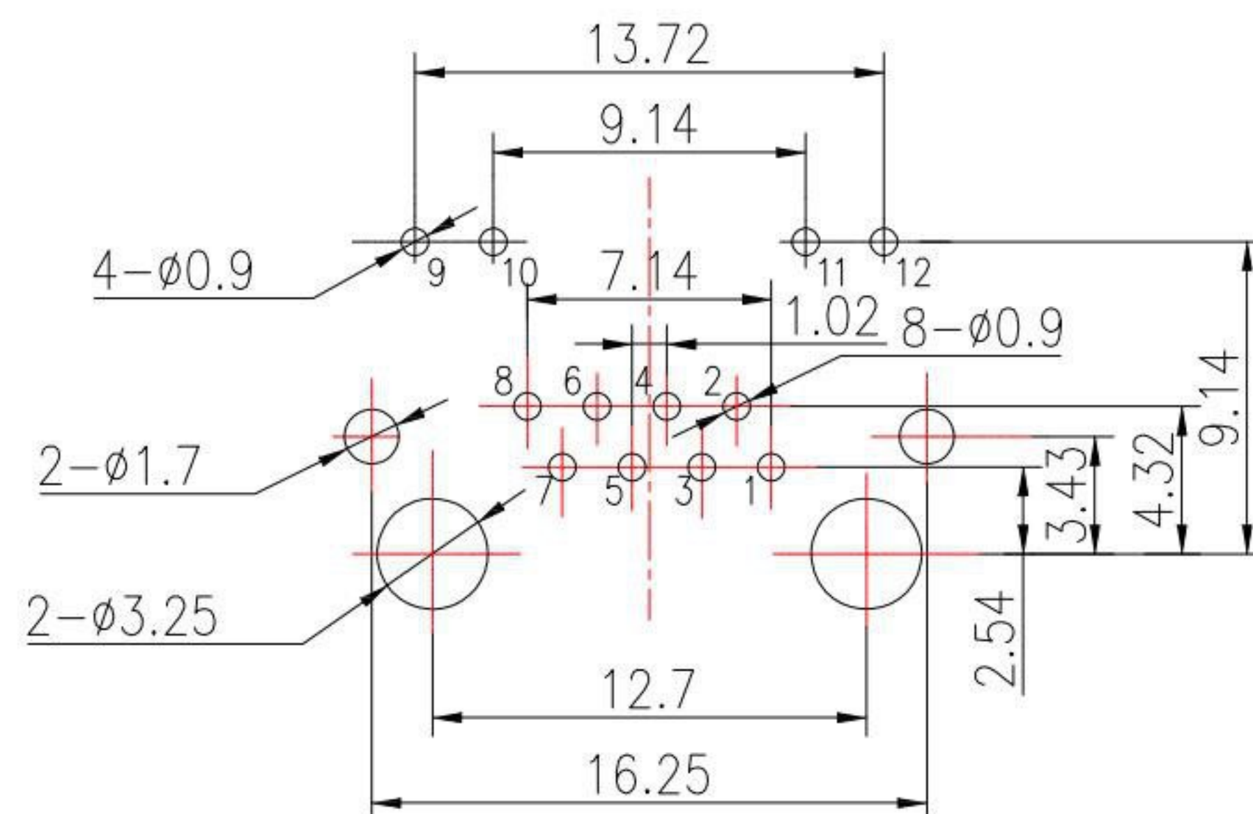
PCB LAYOUT MOUNTING PATTERN
