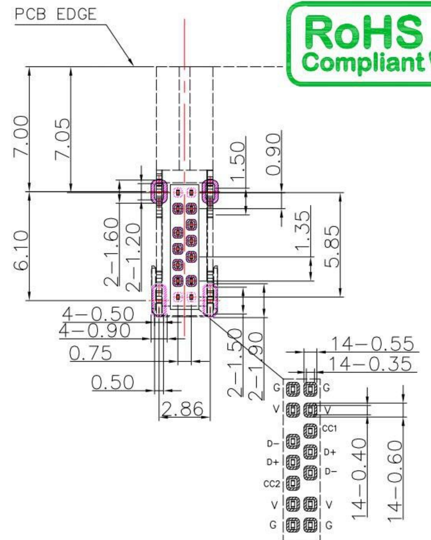
RECOMMENDED P.C.B. LAYOUT
