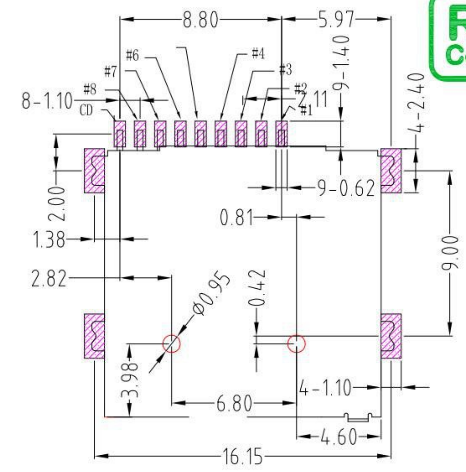
PCB LAYOUT
