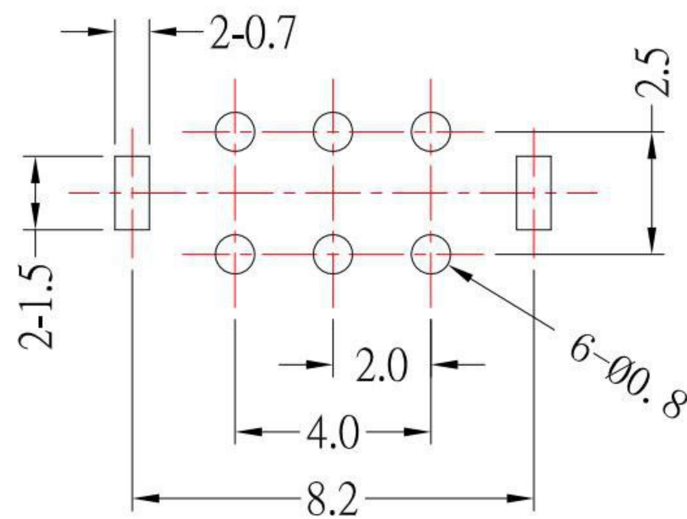
P.C.B LAYOUT BOTTOM VIEW
