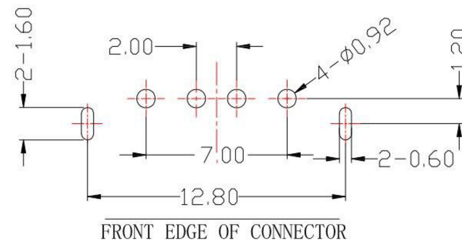
P.C.B LAYOUT MOUNTING PATTERN
