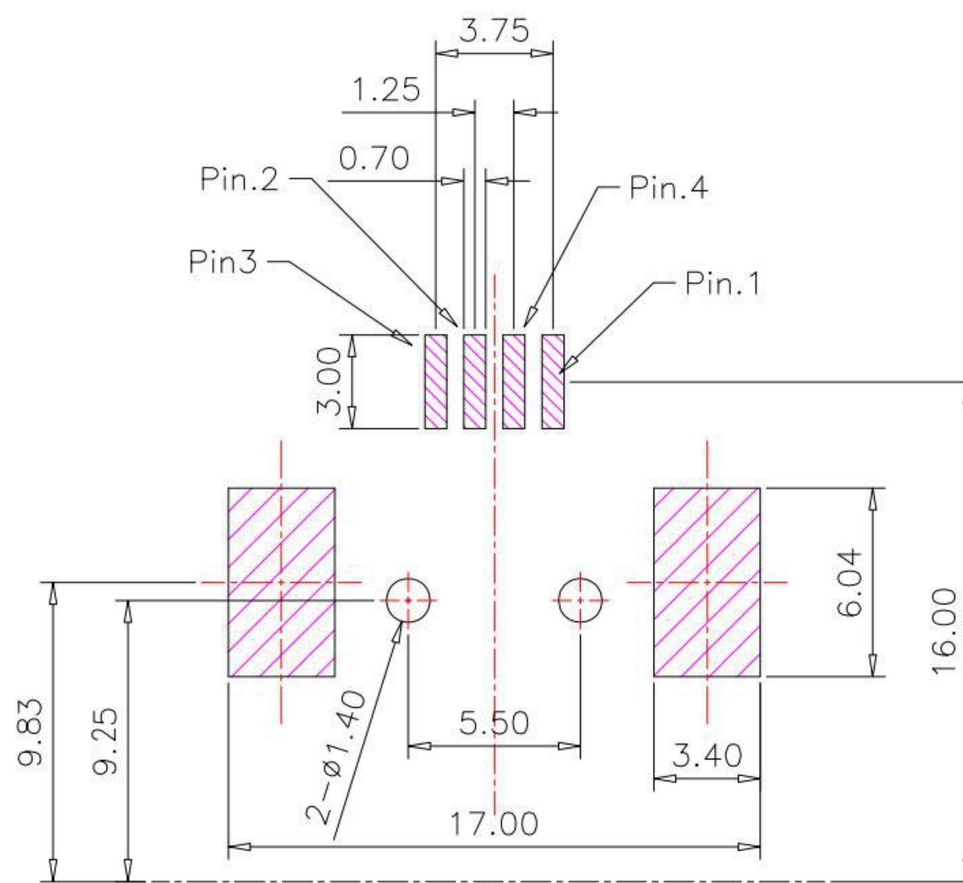
P.C.B LAYOUT MOUNTING PATTERN
