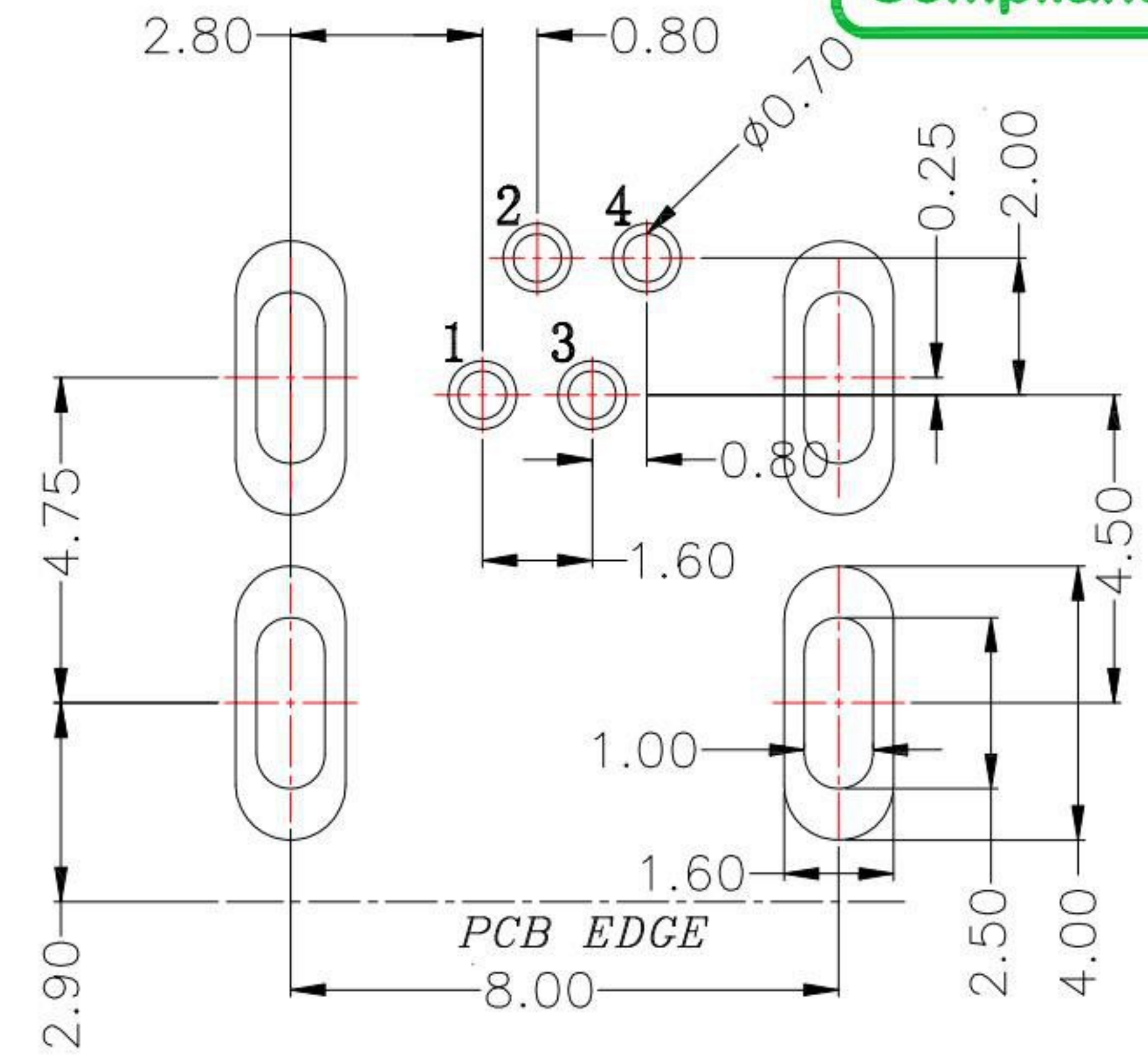
P.C.B LAYOUT MOUNTING PATTERN
