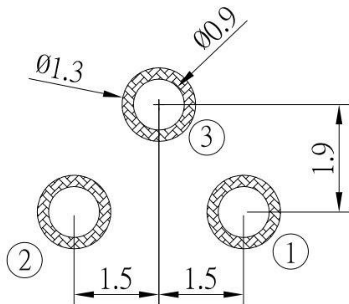
PCB LAYOUT
