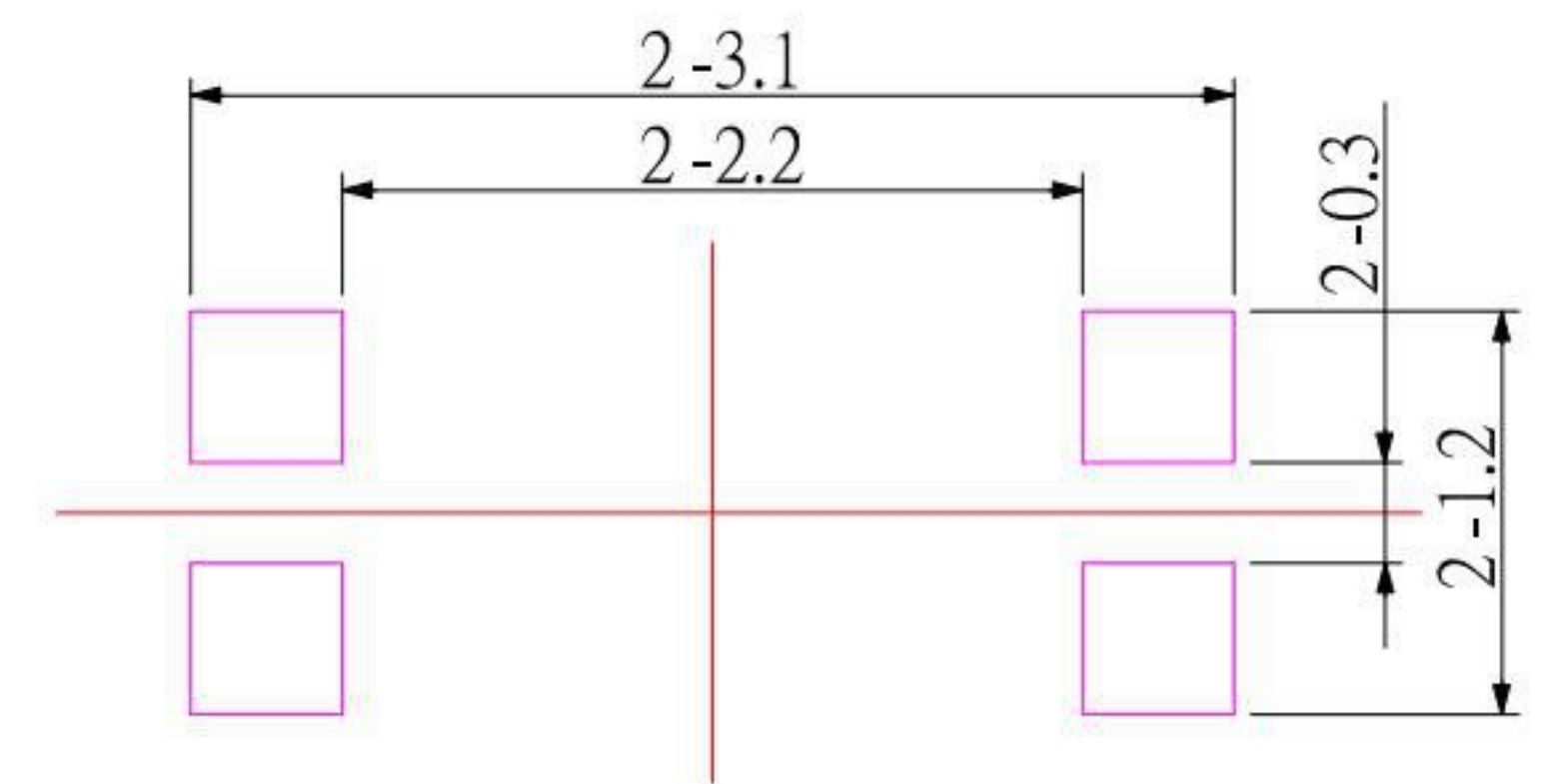
PCB LAYOUT
