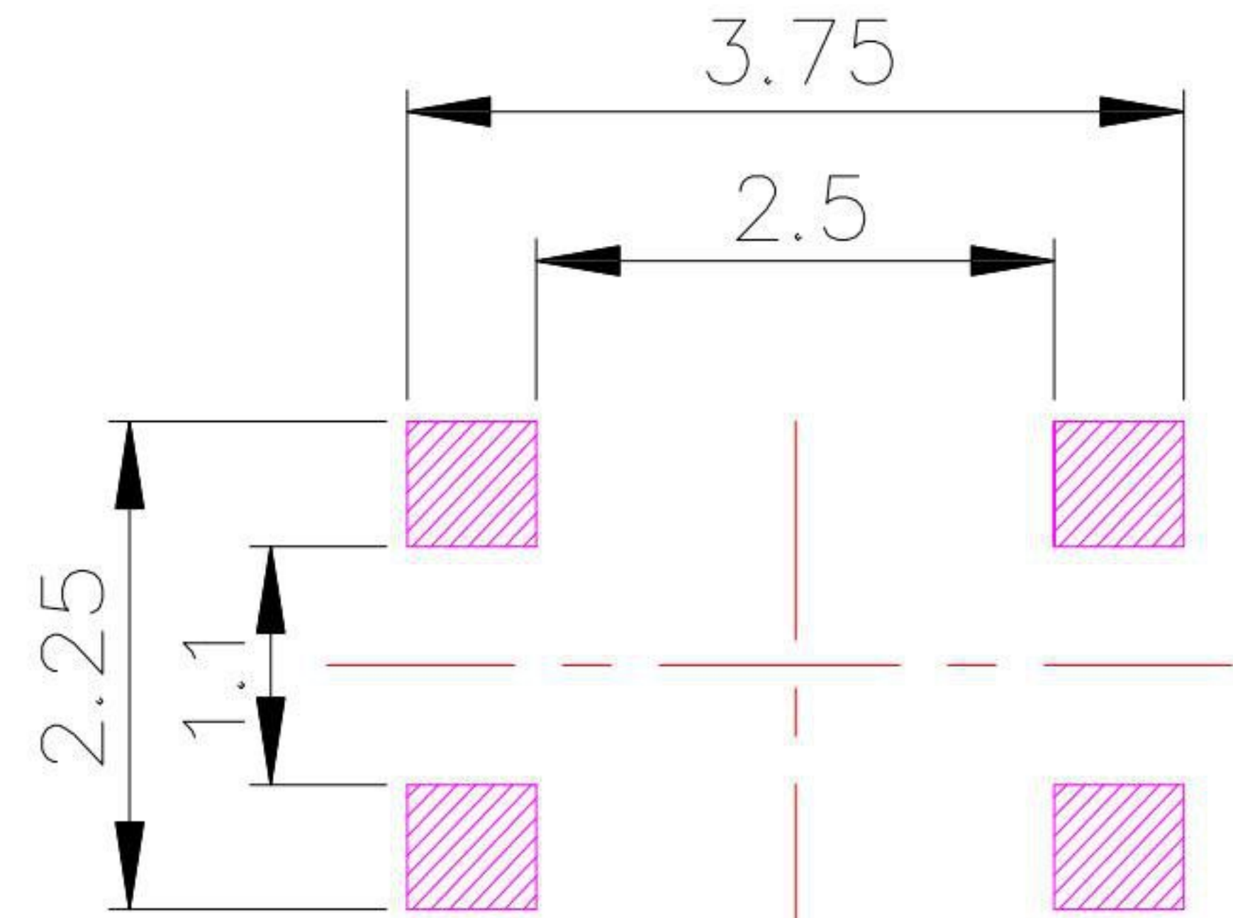
PCB LAYOUT
