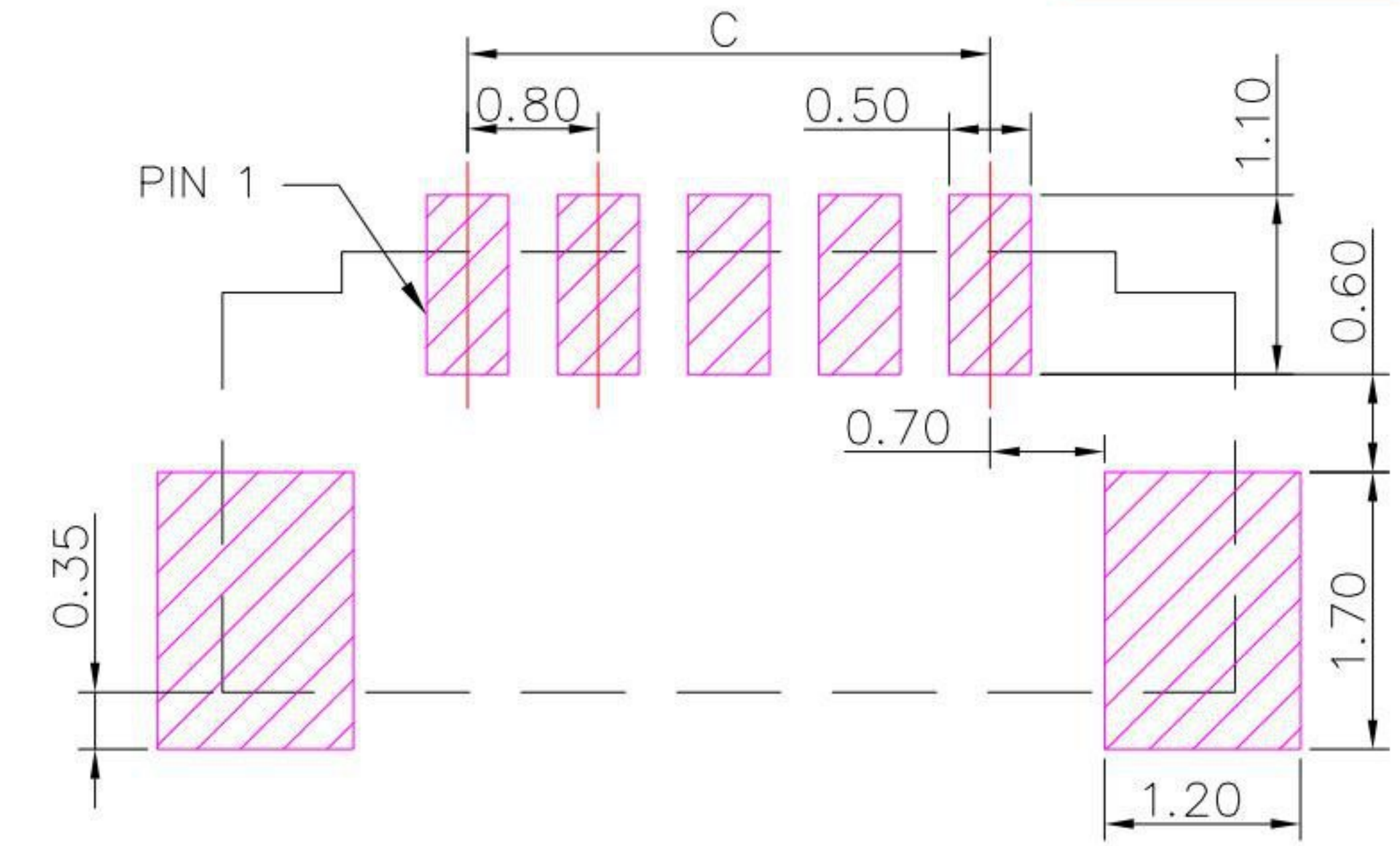
P.C.B LAYOUT MOUNTING PATTERN
