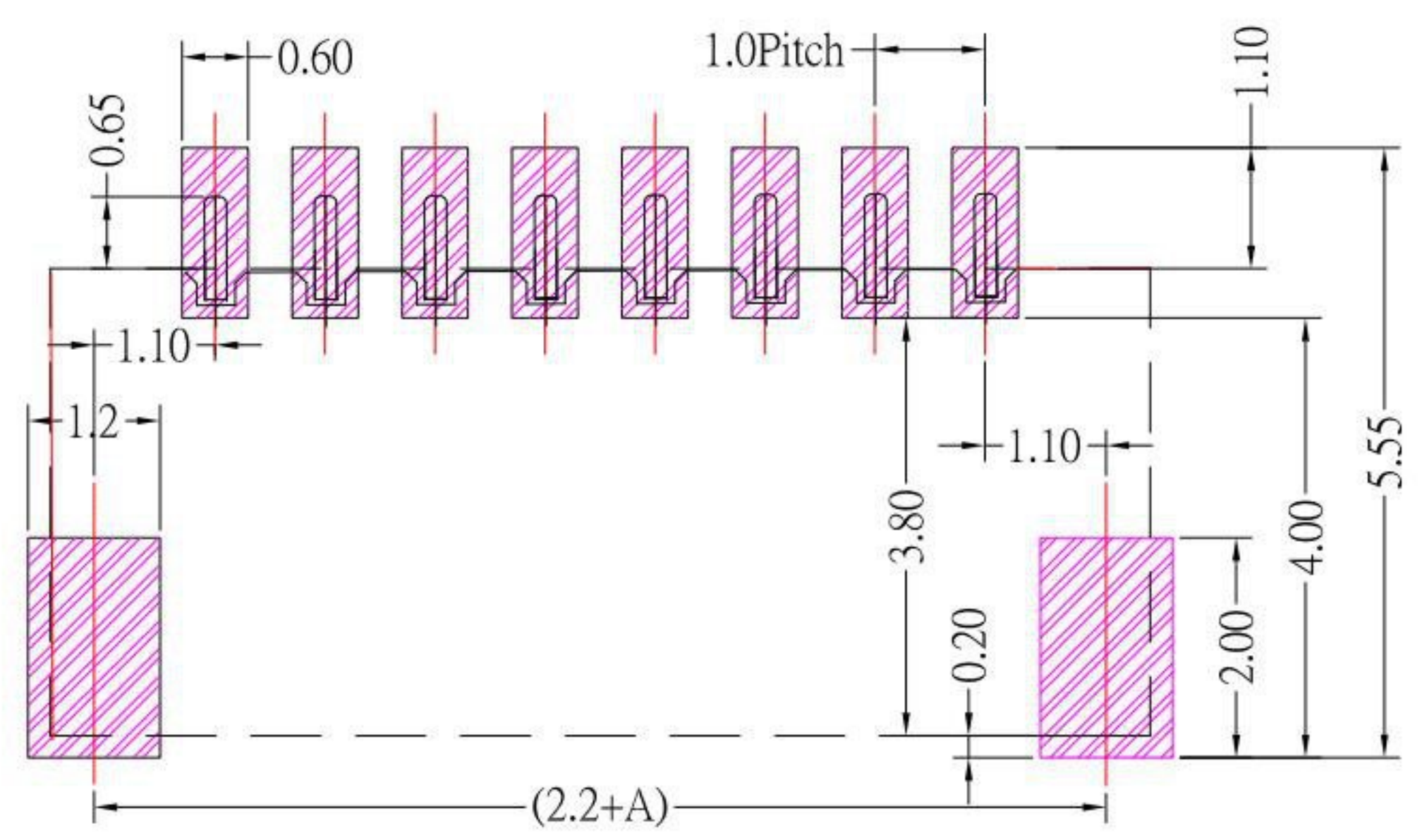
P.C.B LAYOUT MOUNTING PATTERN
