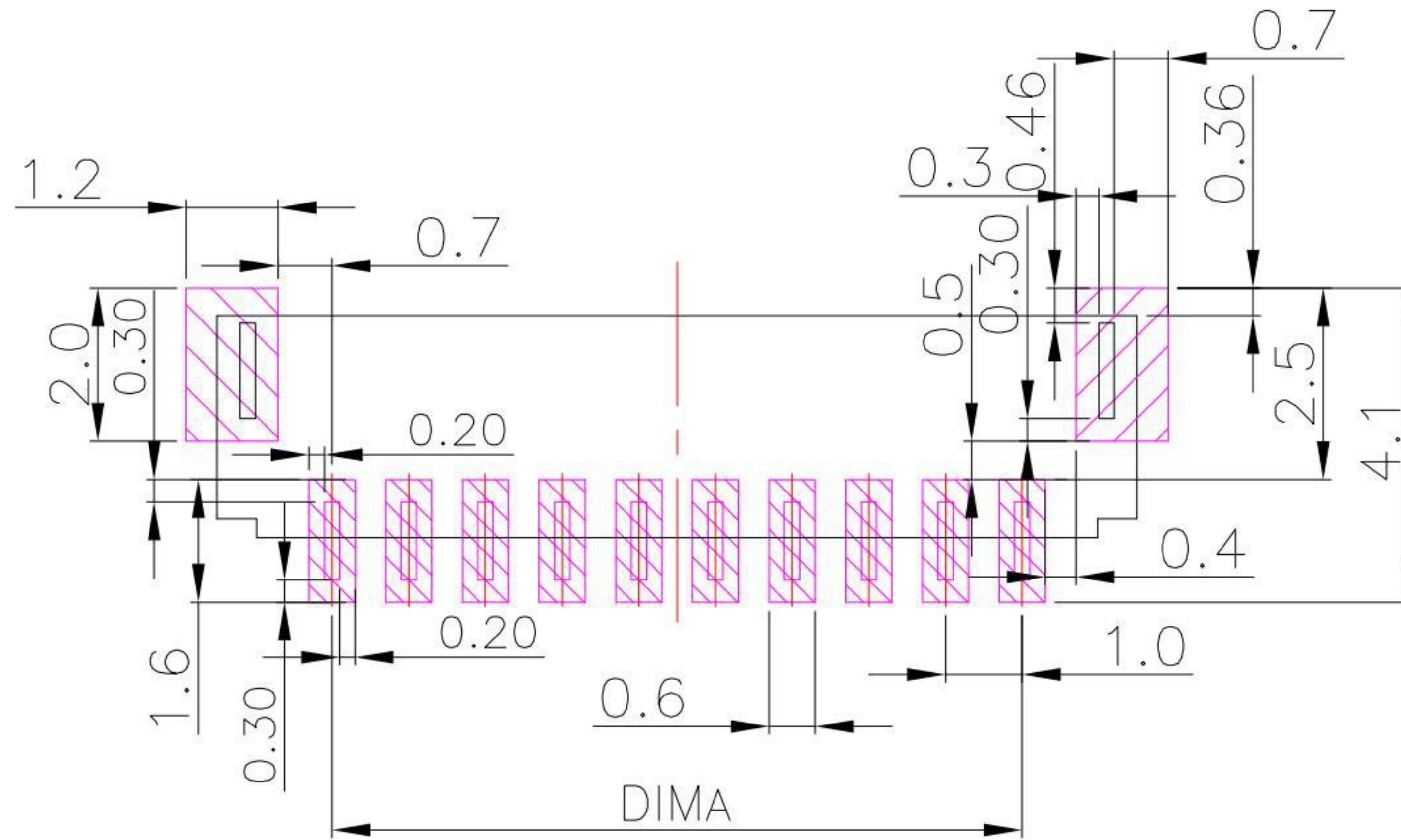
P.C.B LAYOUT MOUNTING PATTERN
