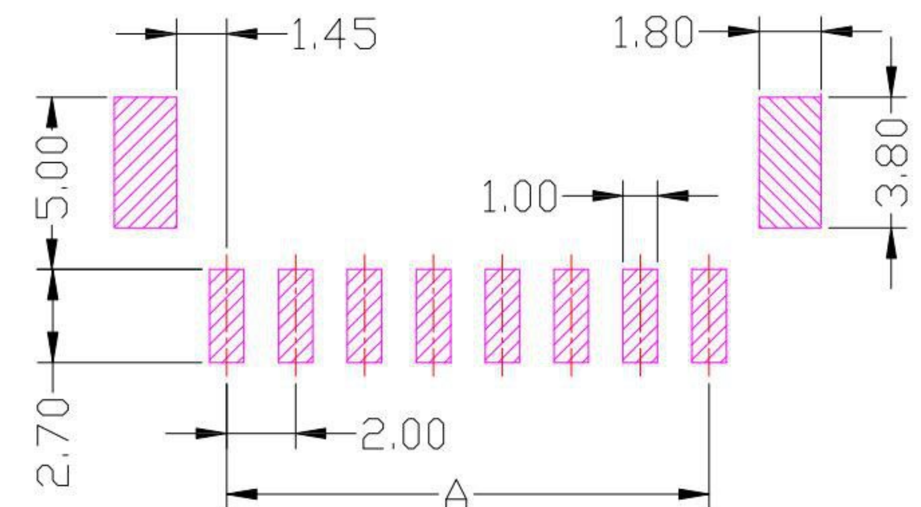
P.C.B LAYOUT MOUNTING PATTERN
