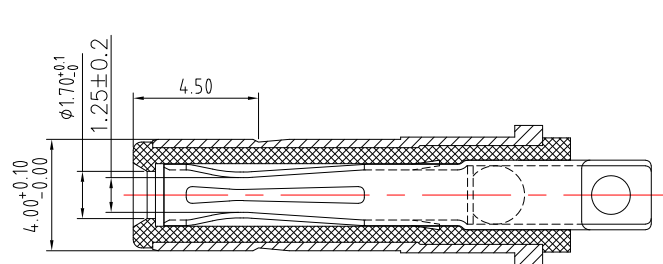
MATING PLUG
