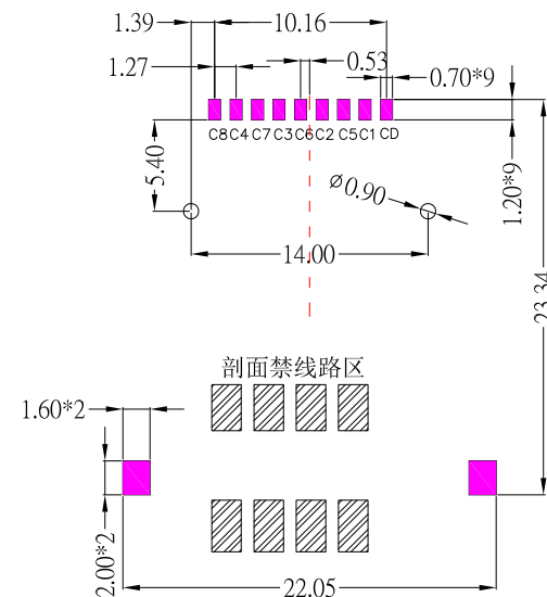
PCB LAYOYT
